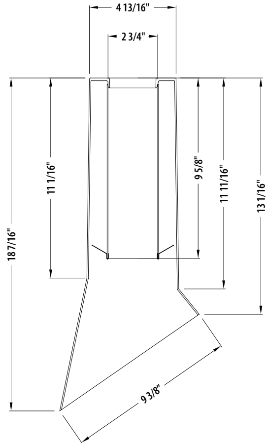
SIDE ELEVATION
